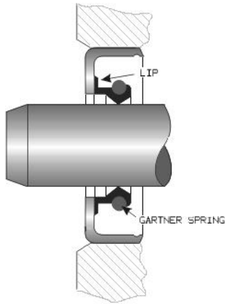
Figure 1. Outline of the seal assembly.
